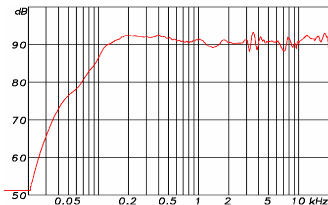
ZL 200 Sens. @ 2, 83V/1m, d=4m
