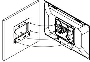
Align mounting frame hooks
